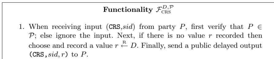
Fig. 2. The Common Reference String functionality
