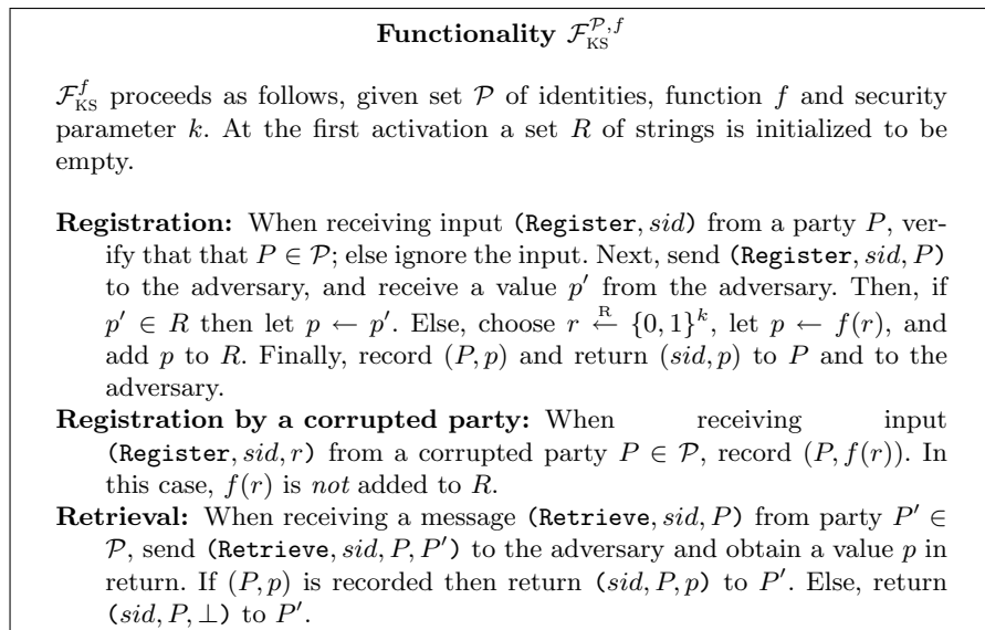
Fig. 3. The Key Registration functionality
